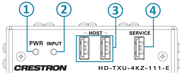
HD-TXU-4KZ-111-E Transmitter, Front Panel
