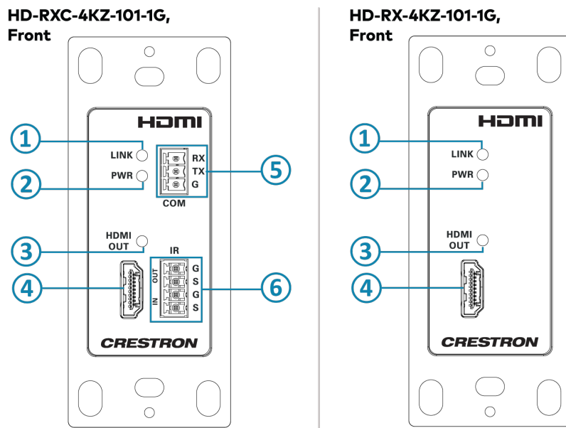
HD-RX(C)-4KZ-101-1G Series Receivers, Front
