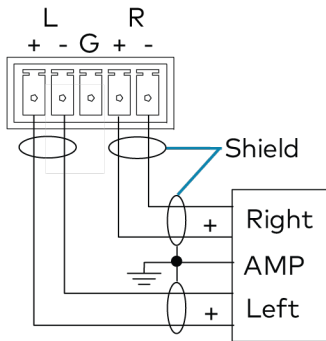
Balanced Output
