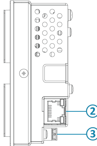
HD-TXU-4KZ-111-2G, Rear, Top View
