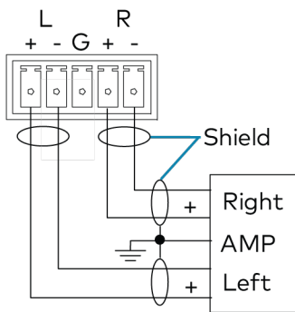
Balanced Output
