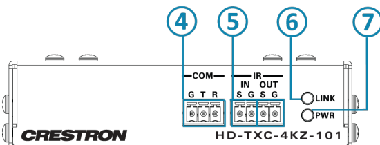
HD-TXC-4KZ-101 Front Panel
