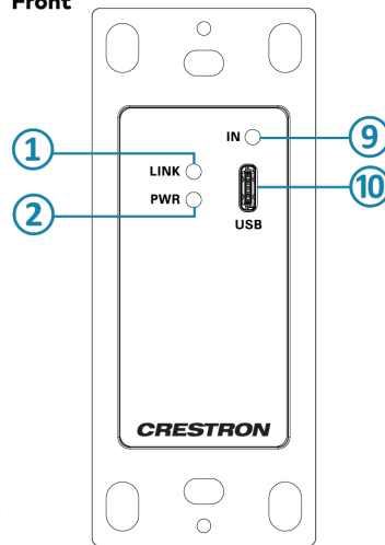
HD-TX-4KZ-111-1G, Front
