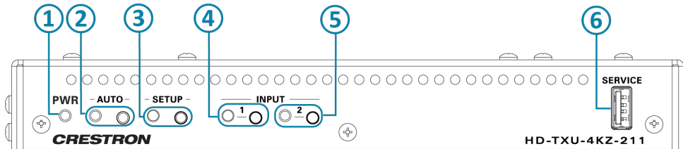
HD-TXU-4KZ-211 Transmitter, Front Panel
