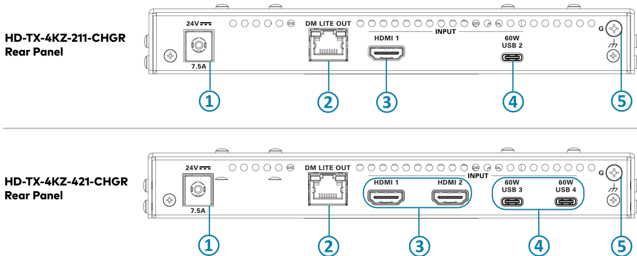
HD-TX-4KZ-211-CHGR and HD-TX-4KZ-421-CHGR Transmitters, Rear Panel
